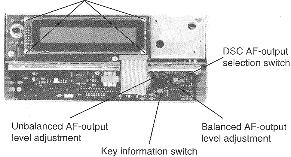
Front view without frontplate Screw for Display section
