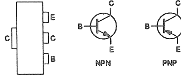
BCP52-16, BCP55-16 (SOT-223 CASE)
