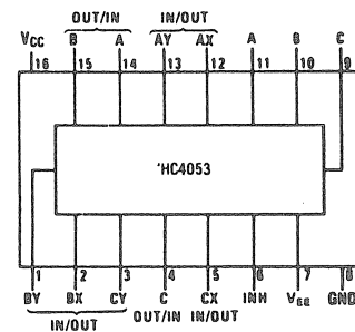
74HC4053 (SO-16 PACKAGE)
