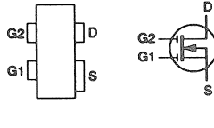
BF996SB (SOT-143 CASE)
