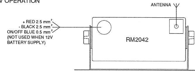
12V OPERATION
