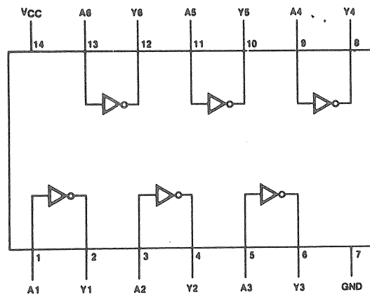
74HC14 (SO-14 PACKAGE)
