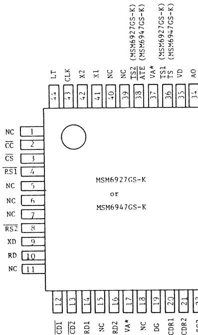
MSM6927 (24-LEAD FLAT-PACK)
