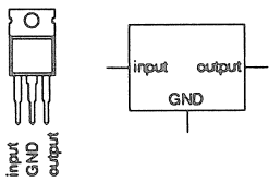
7805 (TO-220 CASE)
