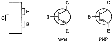
BC848B, BC858B, BFR92A (SOT-23 CASE)
