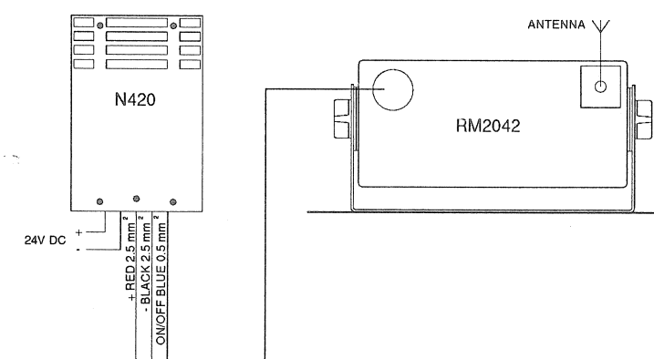
24V OPERATION
