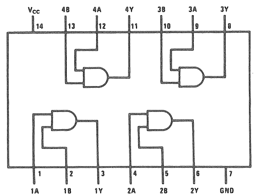
74HC08 (SO-14 PACKAGE)
